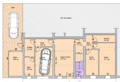
piano terra
